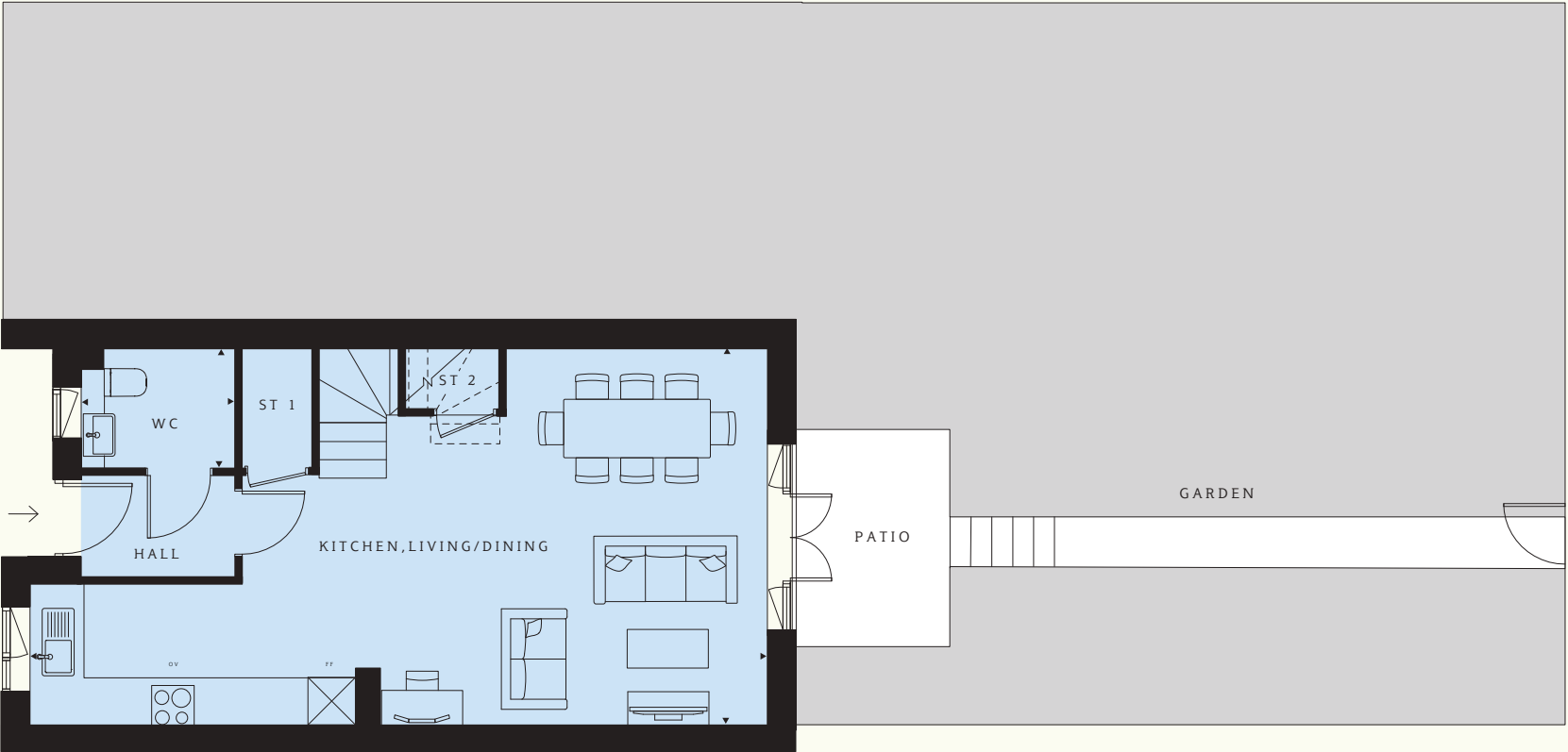
Ground floor
